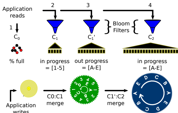
Figure 1: bLSM-Tree architecture
