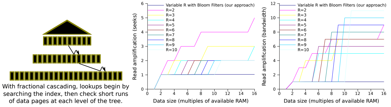
Figure 2: Fractional cascading reduces the cost of lookups from O(\log(n)^2) to O(\log(n)) , but mixes keys and data, increasing read amplification. For our scenarios, Bloom filters’ maximum amplification is 1.03.
